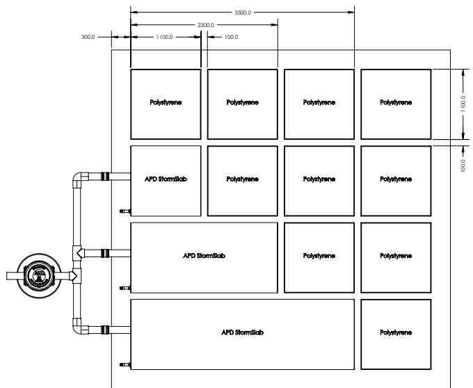
Typical Stormslab layout in "Rib Ruff" Style Concrete Floor Layout
